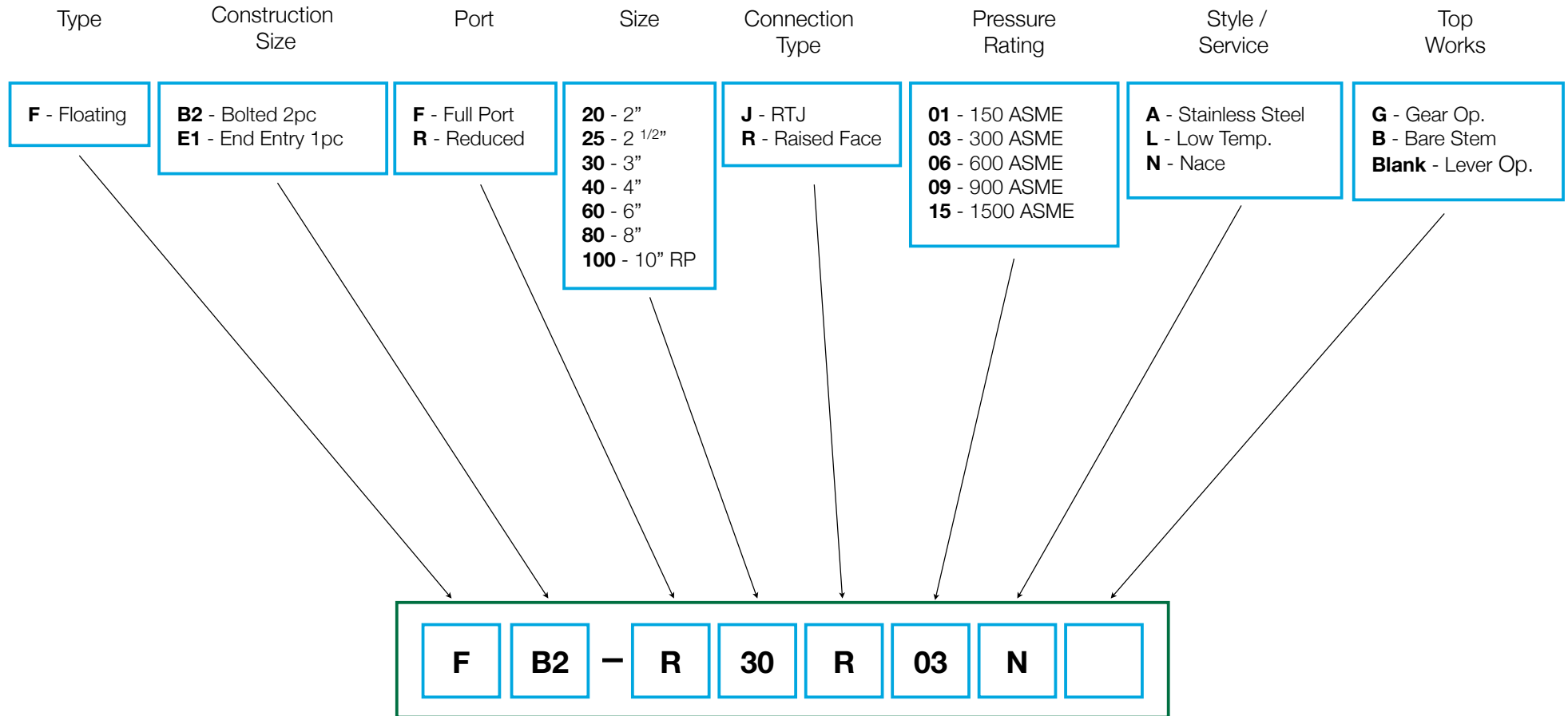
Floating Ball End Entry Bolted 2-Piece, Reduced Port, 3 Inch, Raised Face 300 Class, Nace Trim, Lever Op.
